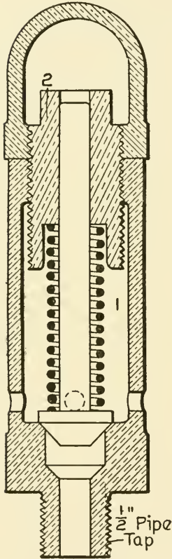
Fig. 97. Section of Safety Valve
